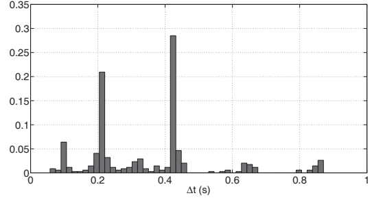
Fig. 2. Probability density estimate of the inter-onset-intervals extracted from the first onset fusion stage.
