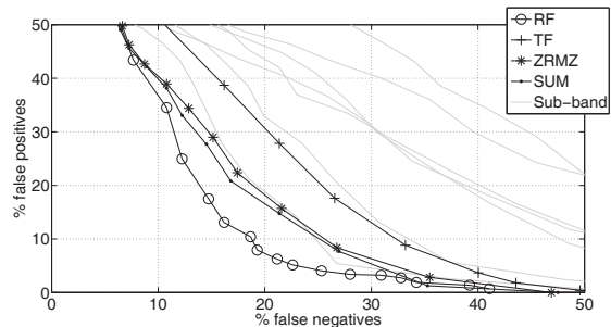
Fig. 3. Comparison of onset detection algorithms: the reference state of the art approach (ZRMZ), the sum of sub-band detection functions (SUM), the individual sub-band onset detection functions (Sub-band) and the temporal (TF) and rhythmic (RF) fusion approaches.
